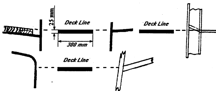
Figure 1: Deck-line
